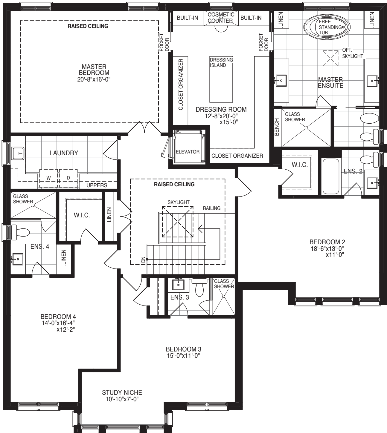
Elevation C SECOND FLOOR
