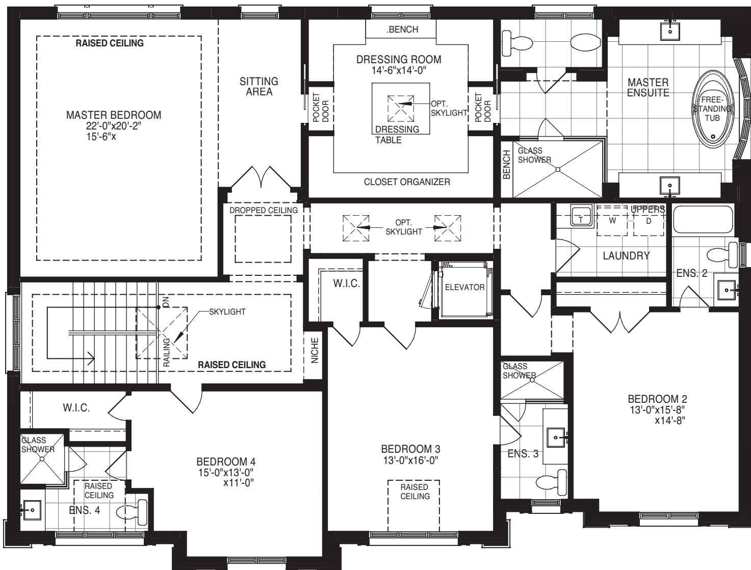
Elevation B SECOND FLOOR
