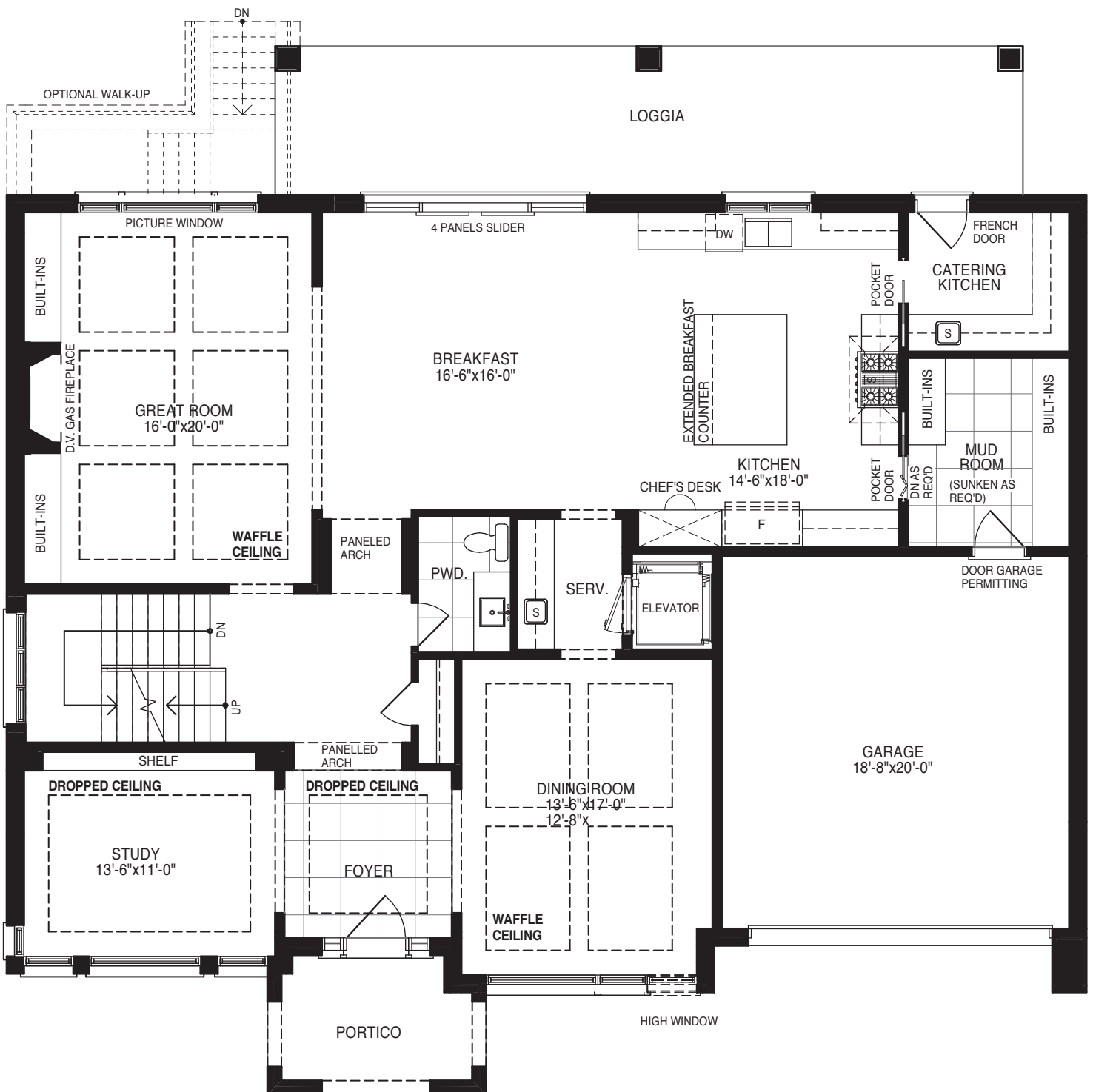
Elevation C GROUND FLOOR
